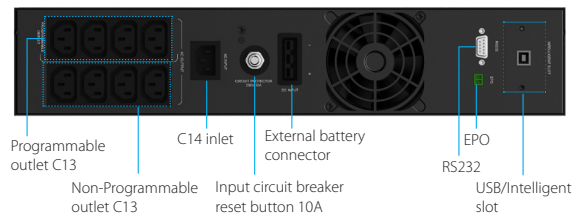
1kVA Rear Panel
