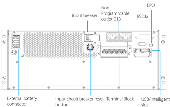
6-10kVA Rear Panel
