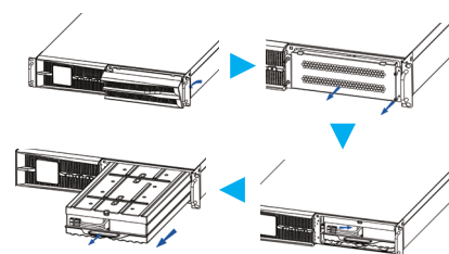
Hotswappable Battery Replacement
