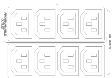
Programmable Outlet(1-3kVA)
